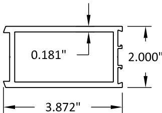
⑩⑦ MEETING STILE (ACTIVE)
