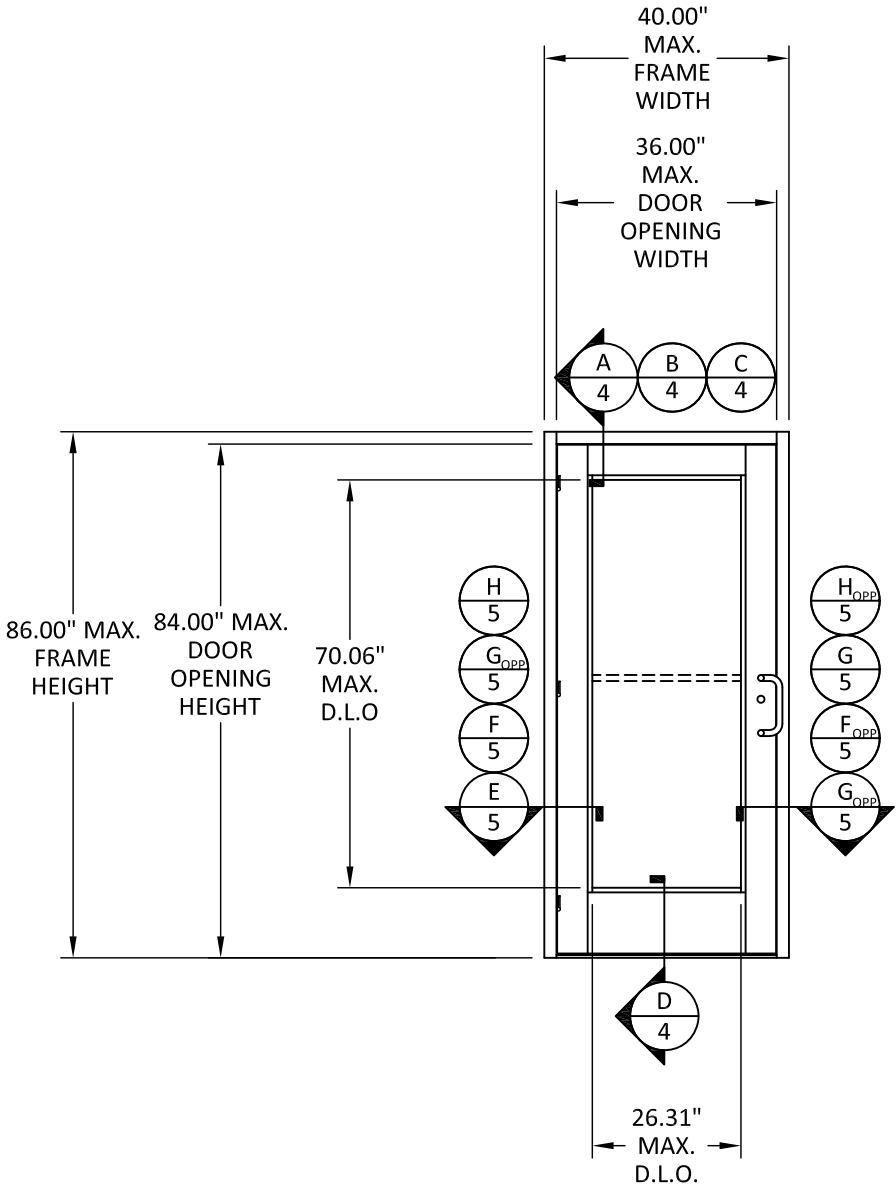
TYPICAL ELEVATION OUTSWING DOOR
