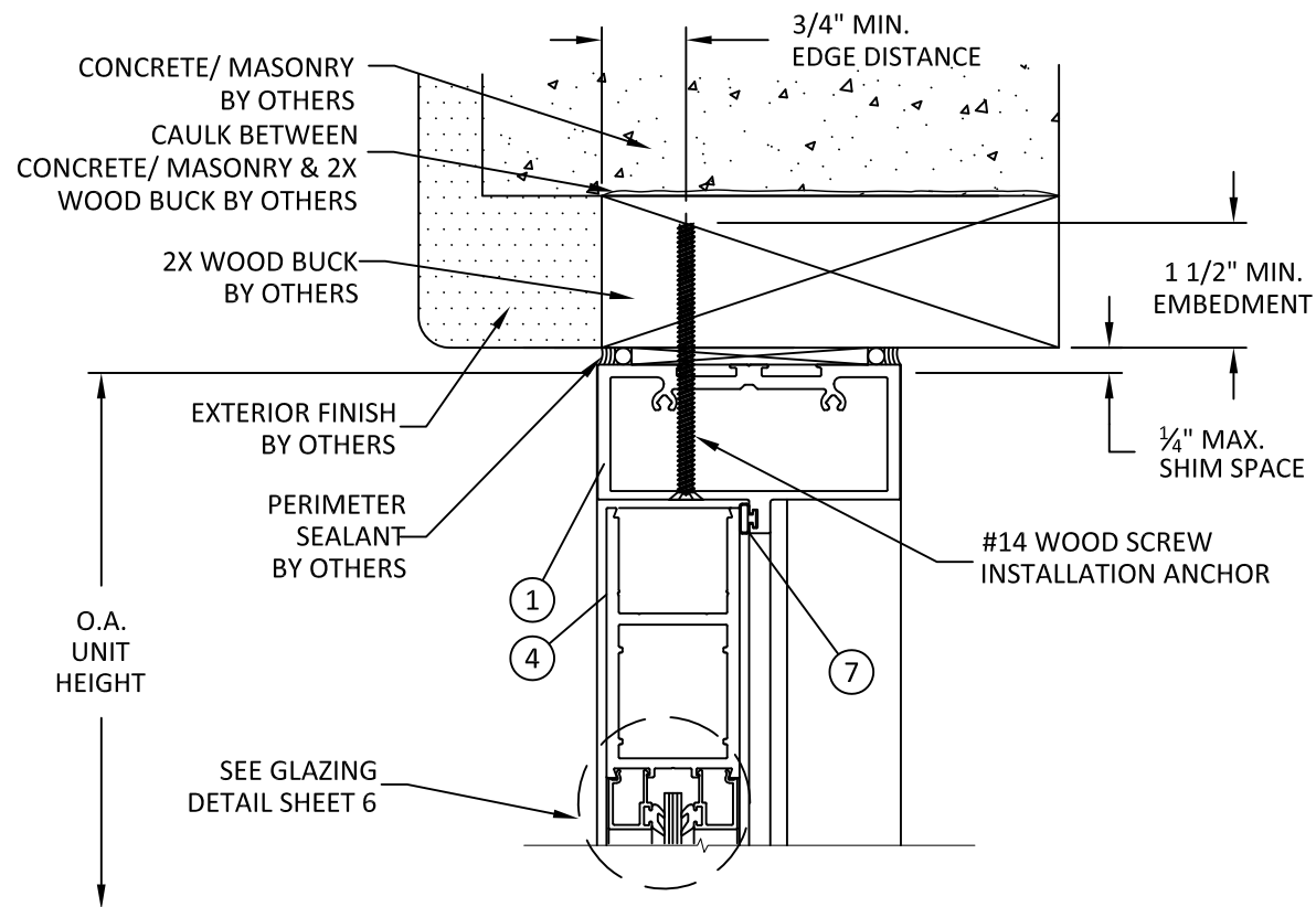
A 4 VERTICAL SECTION DOOR HEAD - 2X WOOD BUCK THROUGH FRAME
