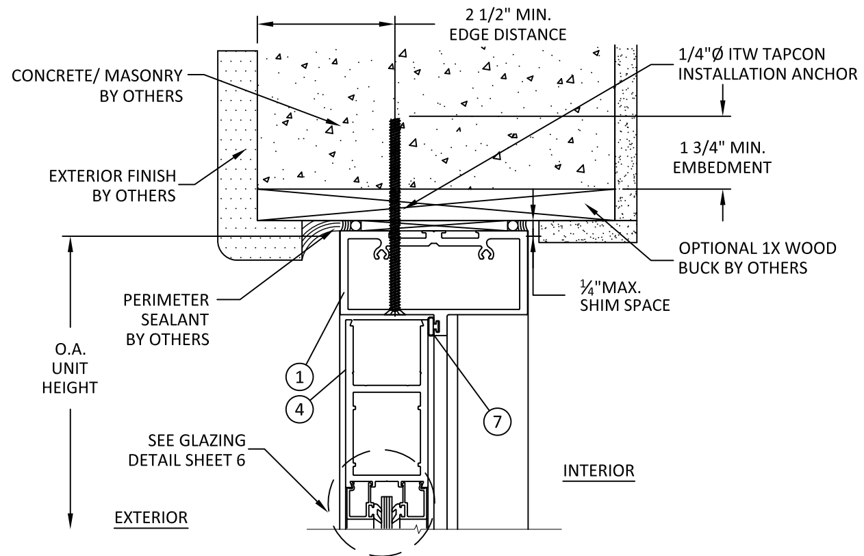
B 4 VERTICAL SECTION DOOR HEAD - CONCRETE/MASONRY THROUGH FRAME
