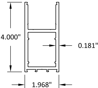
④ 4" TOP RAIL
