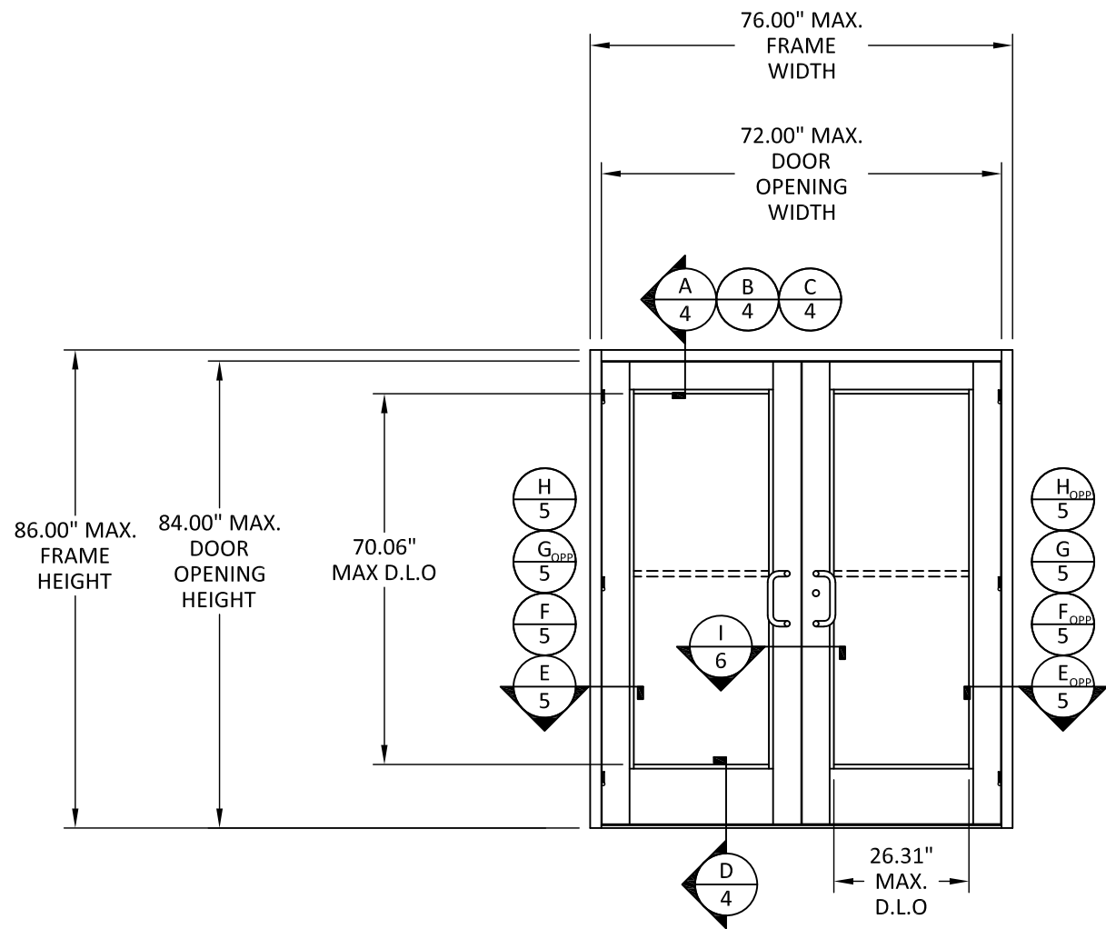
TYPICAL ELEVATION OUTSWING DOOR
