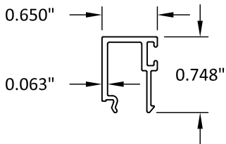
⑩ 1/4" GLASS STOP
