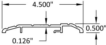
⑩③ 4-1/2" DOOR THRESHOLD
