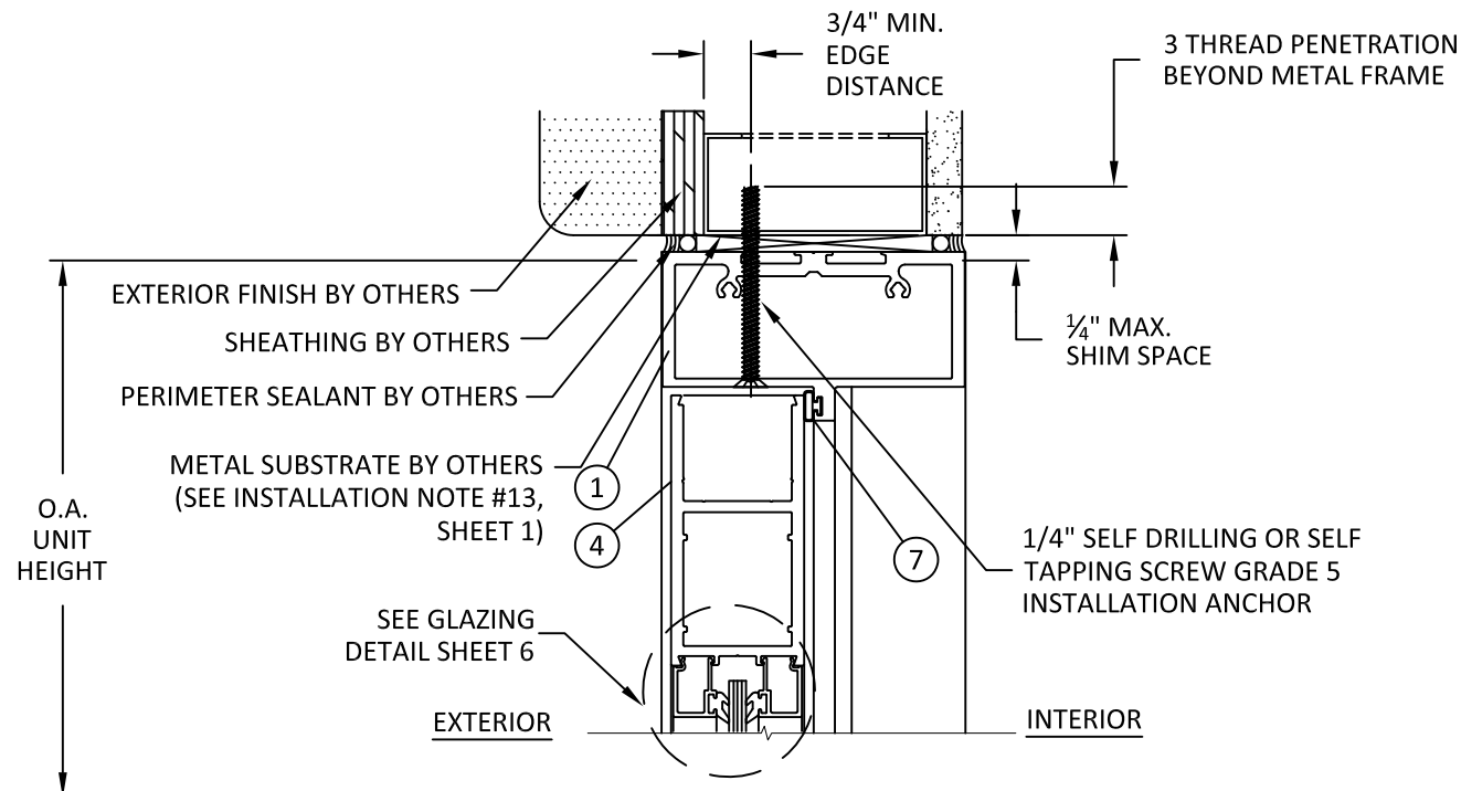
C 4 VERTICAL SECTION DOOR HEAD - STEEL STUD/ALUMINUM MULLION THROUGH FRAME
