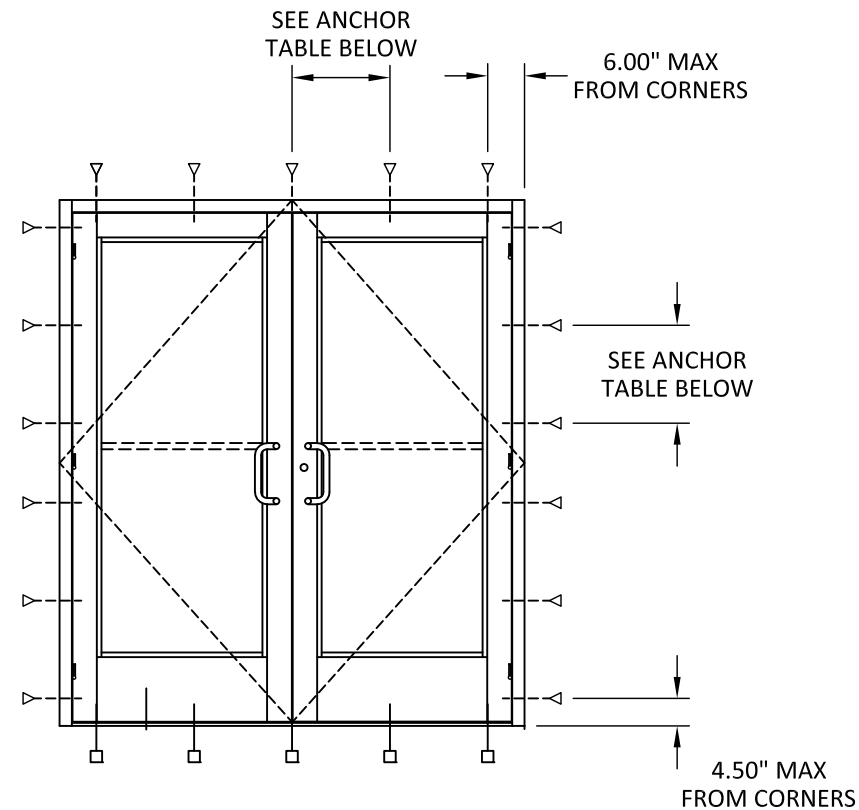
ANCHOR LAYOUT OUTSWING DOOR
