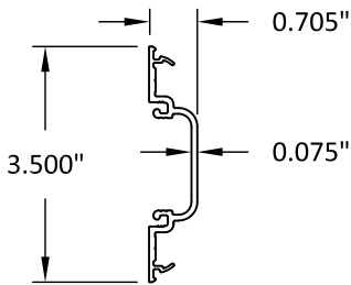
⑩②① SHALLOW POCKET FILLER
